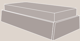
1 SOMMIER / BOX SPRING (80x190) L202 x P100 x H38 (90x200) L212 x P110 x H38
